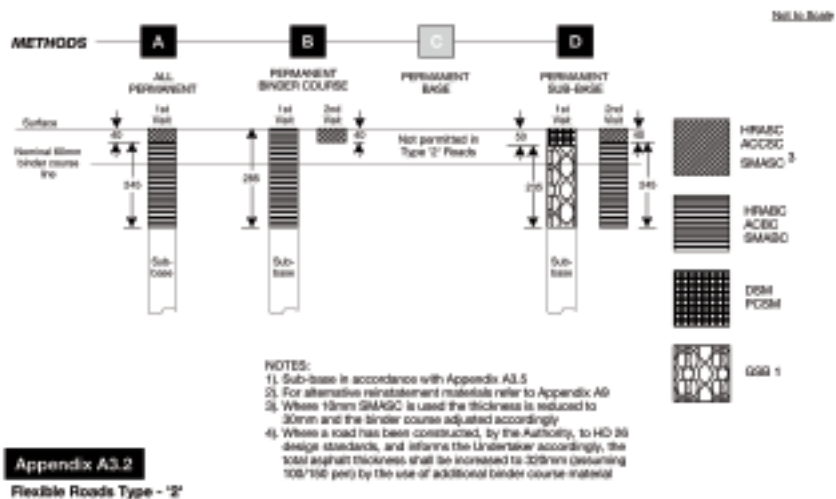
Figure A3.2 Flexible Roads Type - '2'
