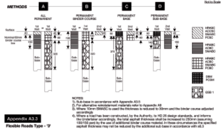
Figure A3.3 Flexible Roads Type - '3'
