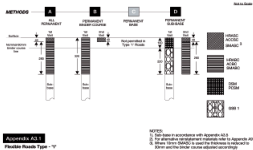
Figure A3.1 Flexible Roads Type - '1'
