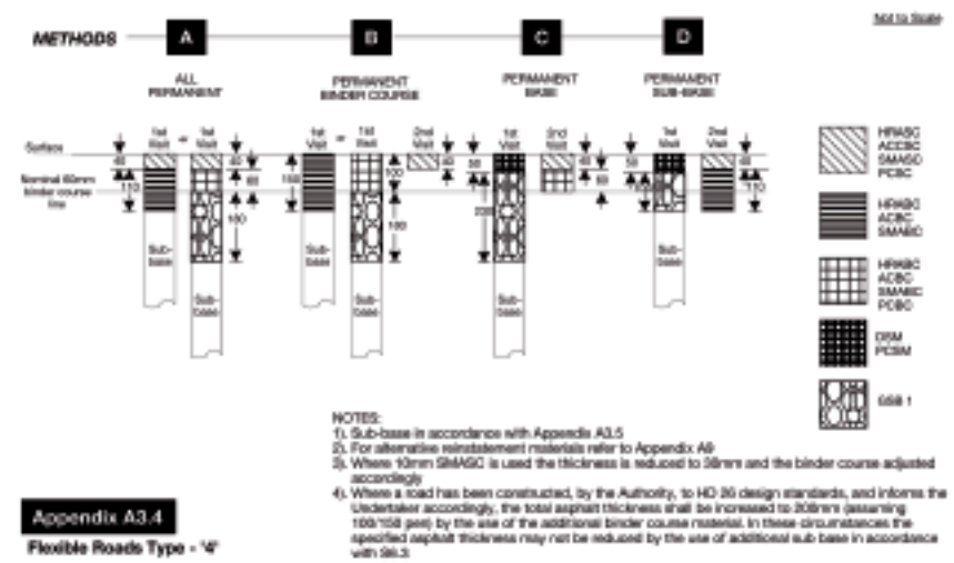
Figure A3.4 Flexible Roads Type - '4'
